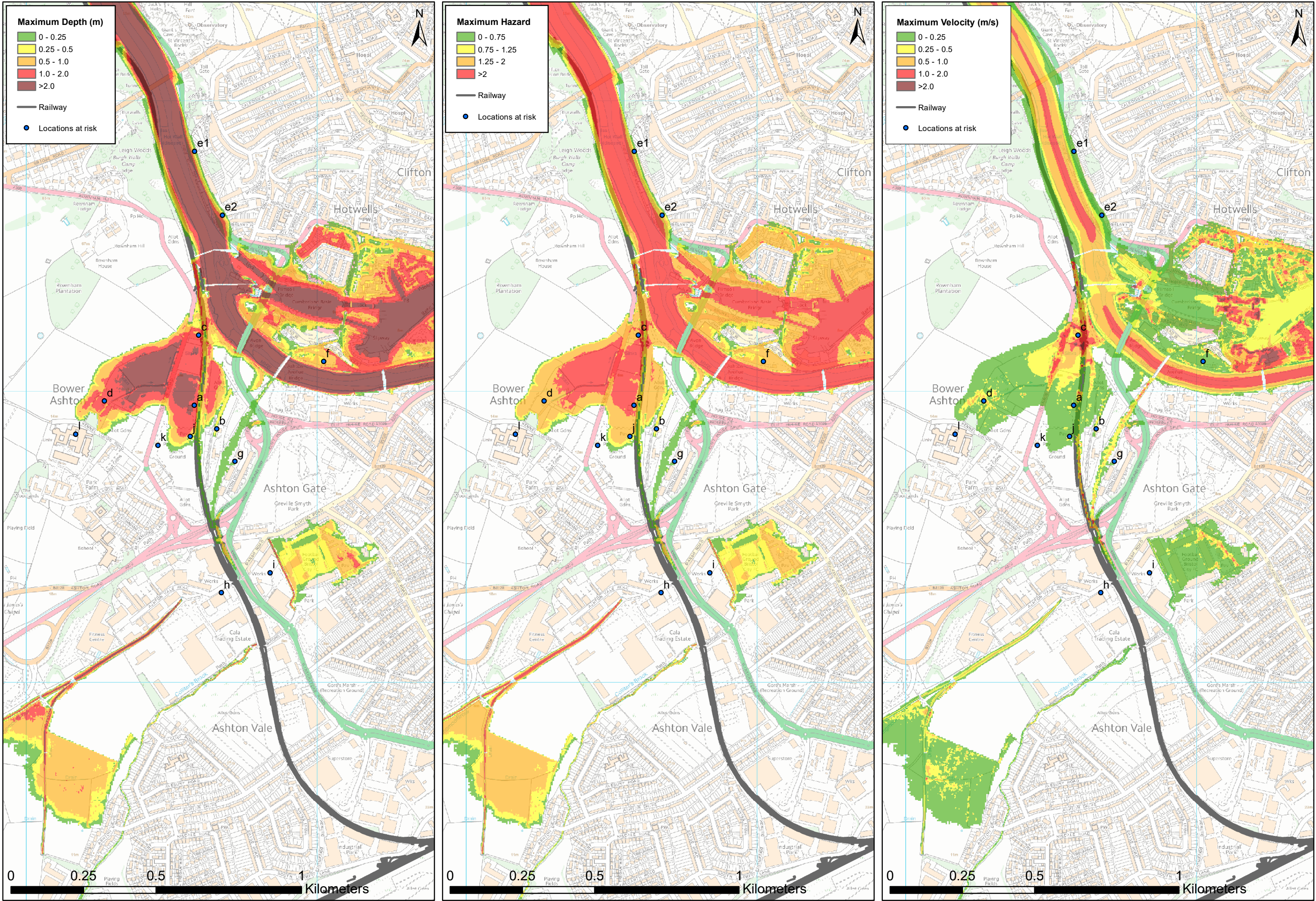
Figure N-18: Post Development, 200year return period event in 2075 ,Tidal
