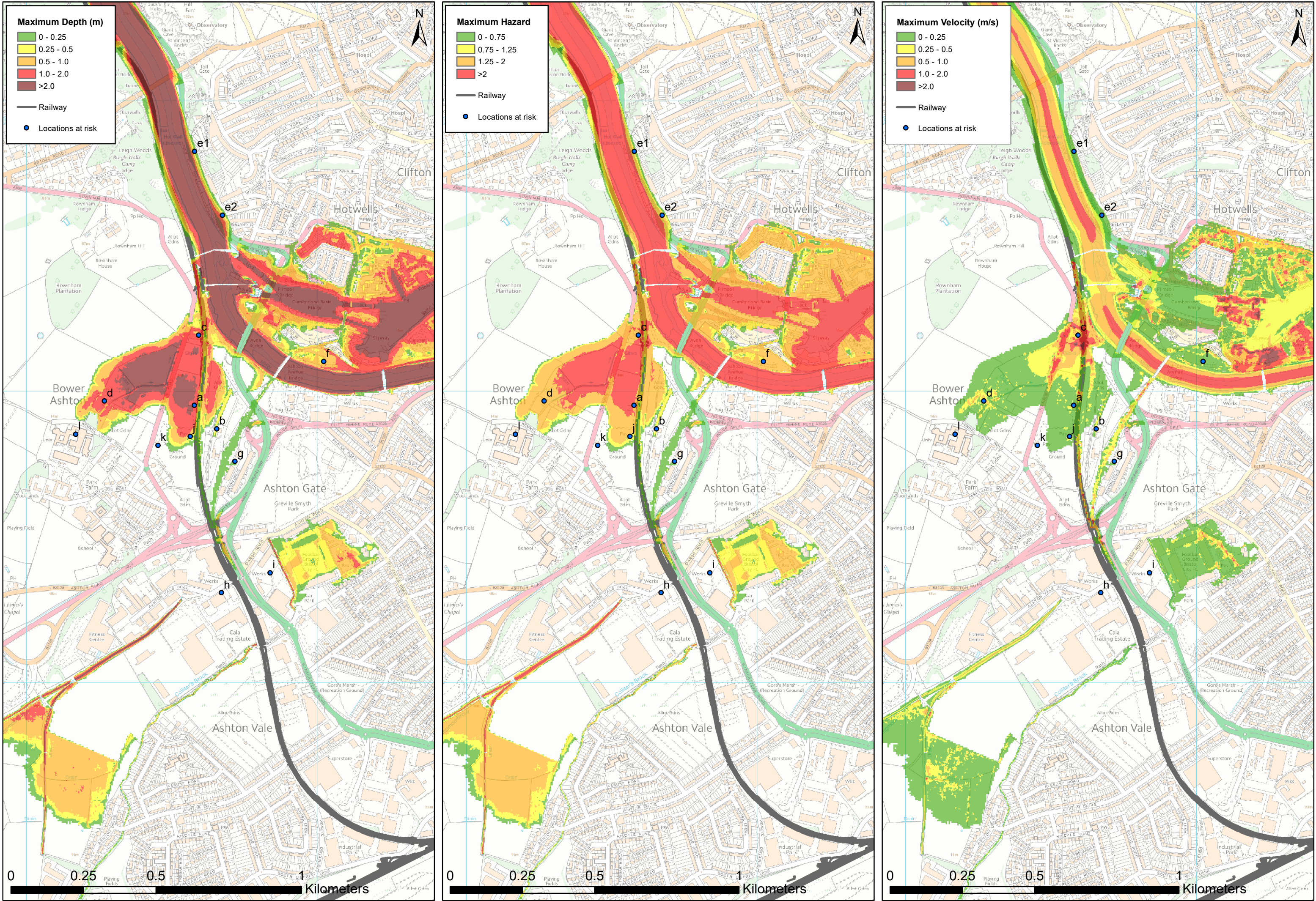
Figure N-17: Pre Development, 200year rerturn period event in 2075 ,Tidal
