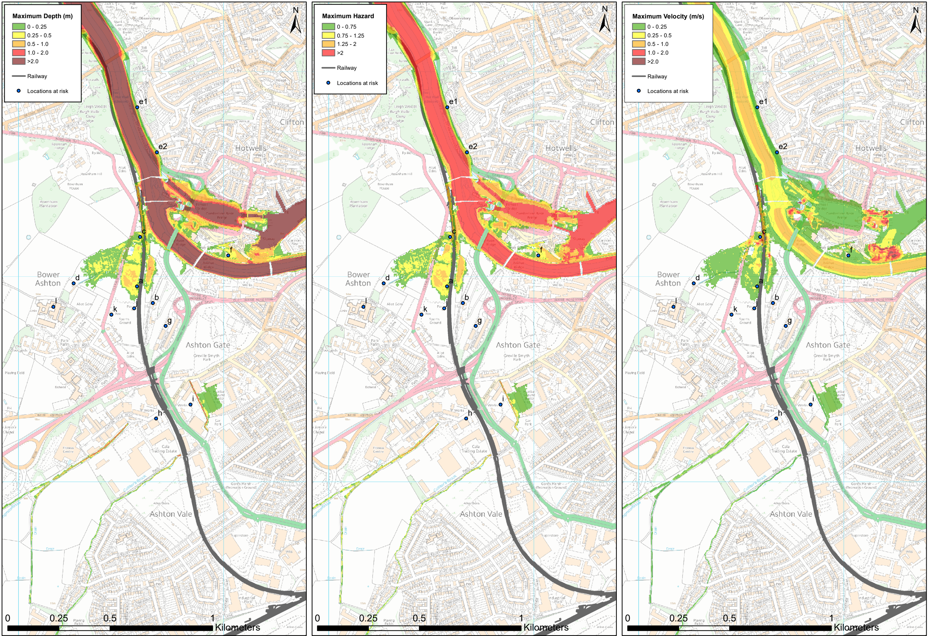
Figure N-11: Pre Development, 10year return period event in 2075 ,Tidal
