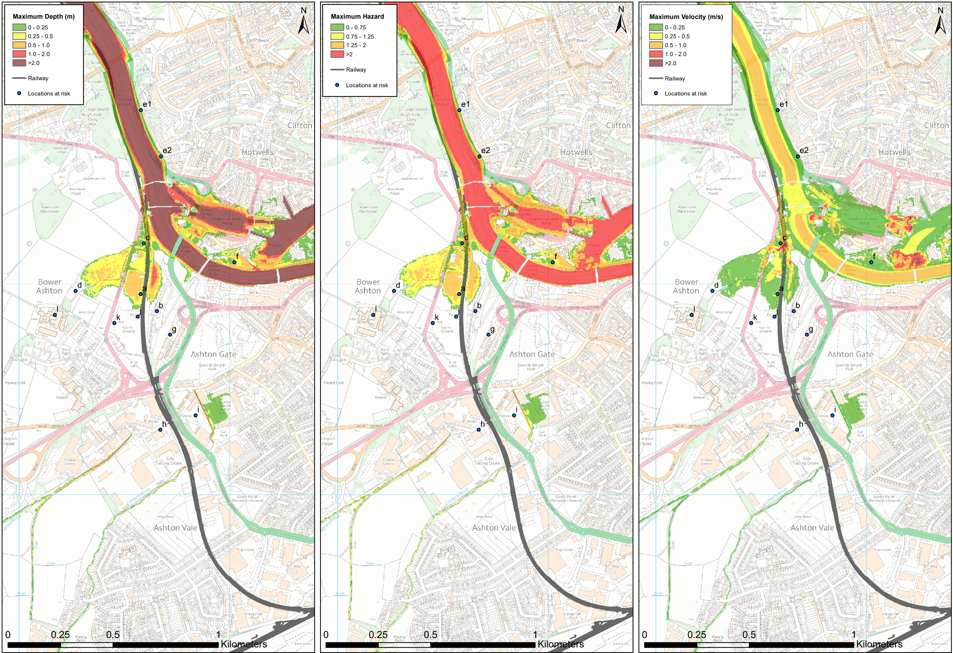
Figure N-14: Post Development, 20year rertun period event in 2075 ,Tidal
