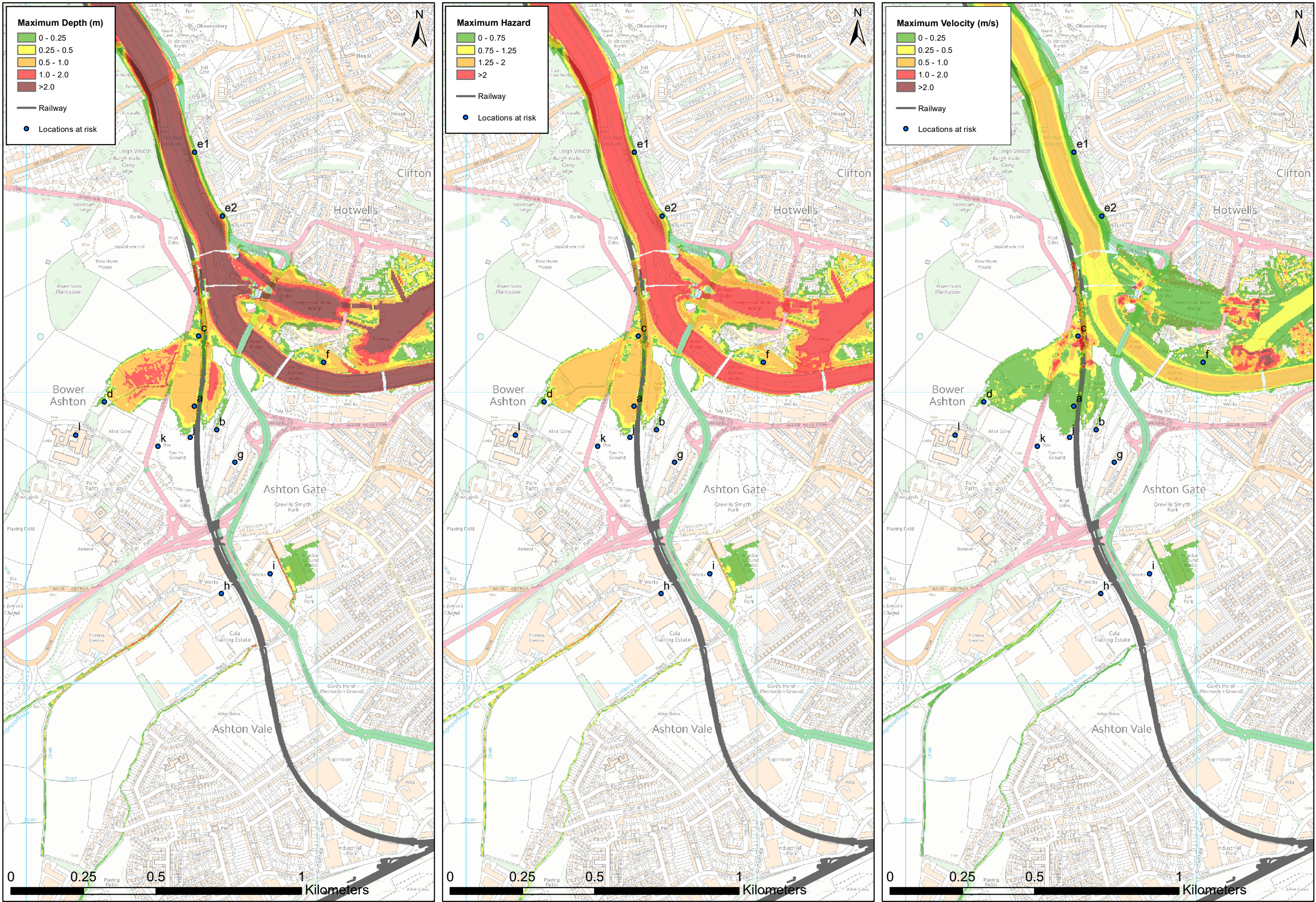
Figure N-15: Pre Development, 75year return period event in 2075 ,Tidal
