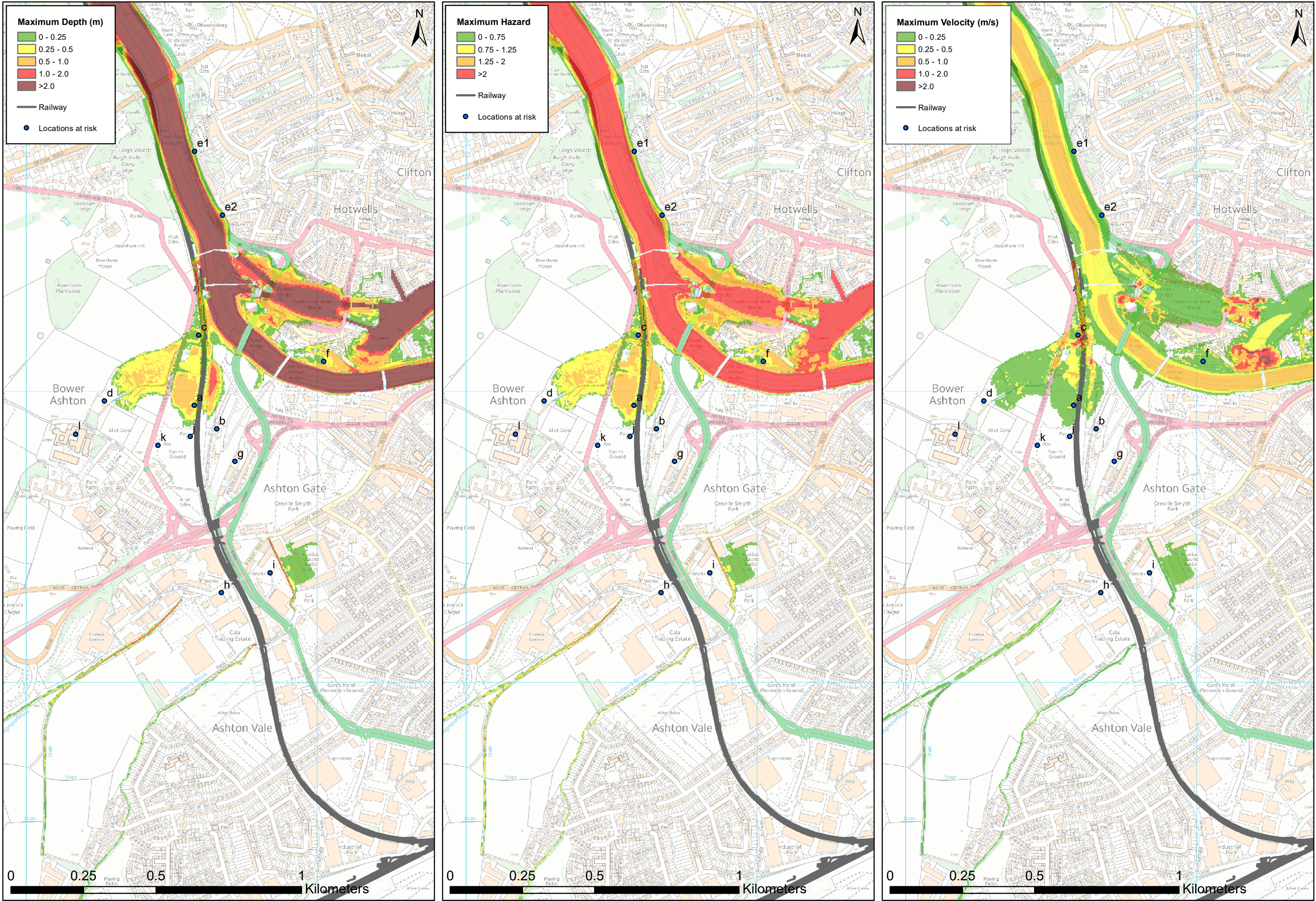
Figure N-13: Pre Development, 20year return period event in 2075 ,Tidal
