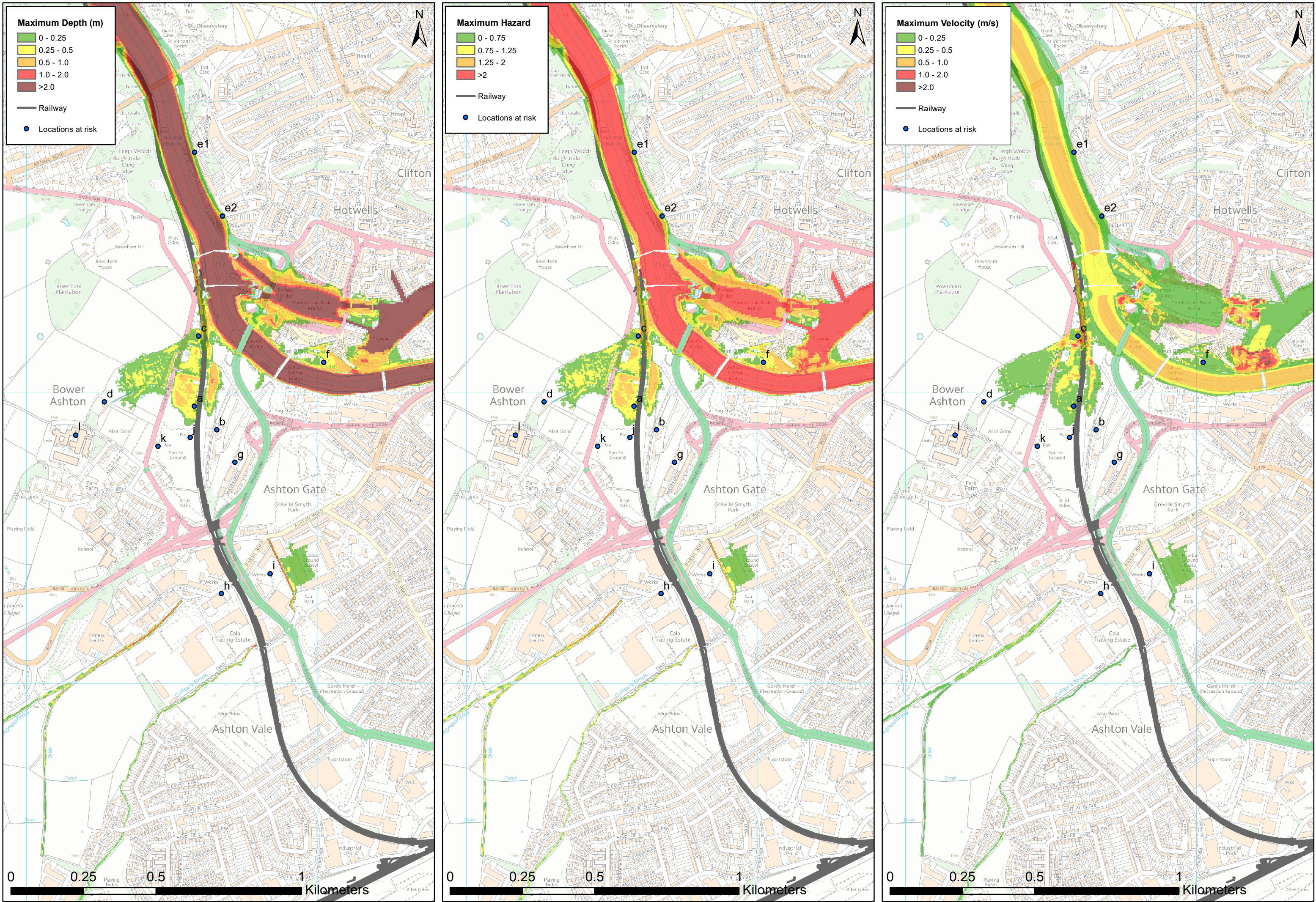
Figure N-12: Post Development, 10year return period event in 2075 ,Tidal
