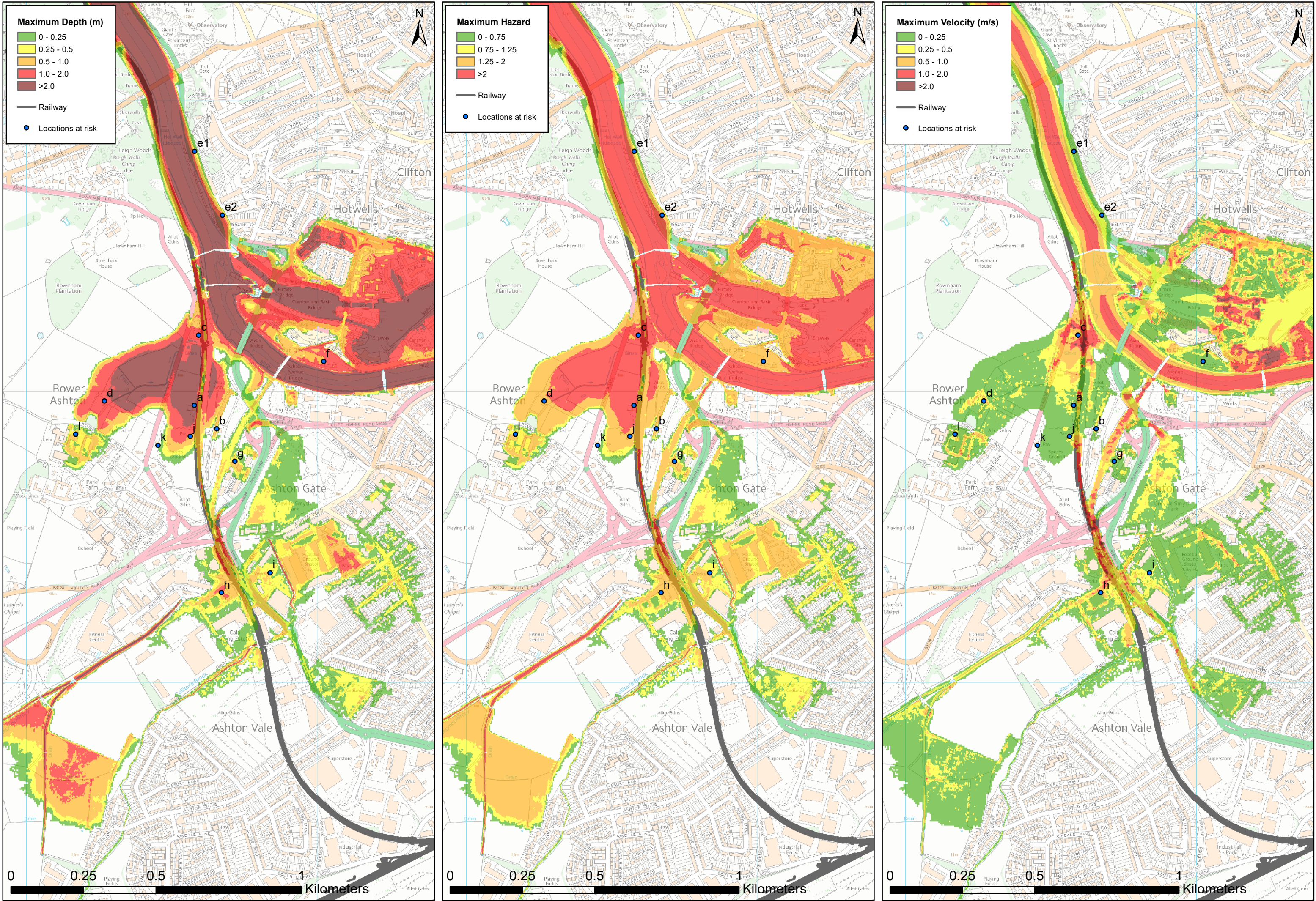
Figure N-19: Pre Development, 1000year return period event in 2075 ,Tidal
