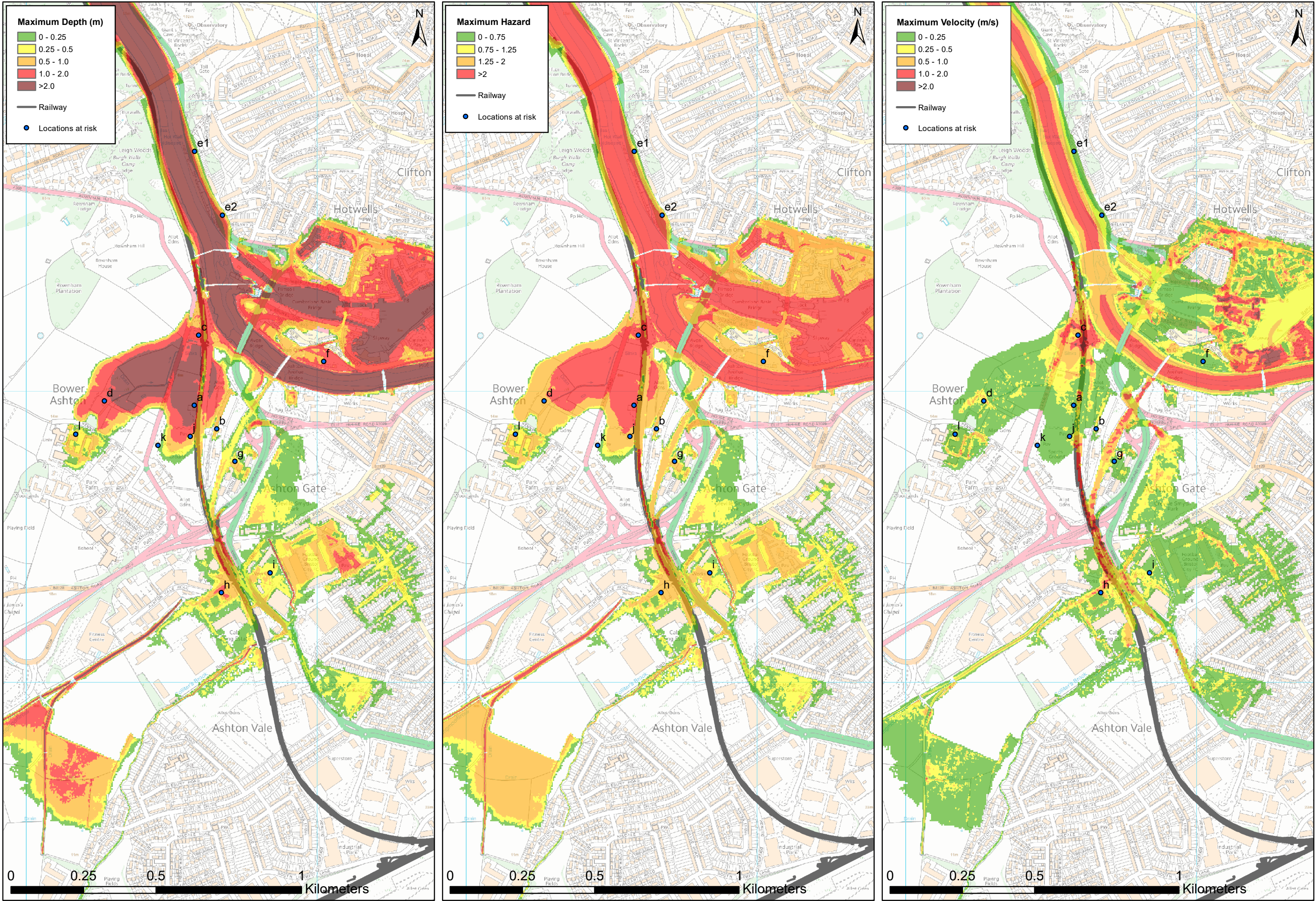
Figure N-20: Post Development, 1000year rerturn period event in 2075 ,Tidal
