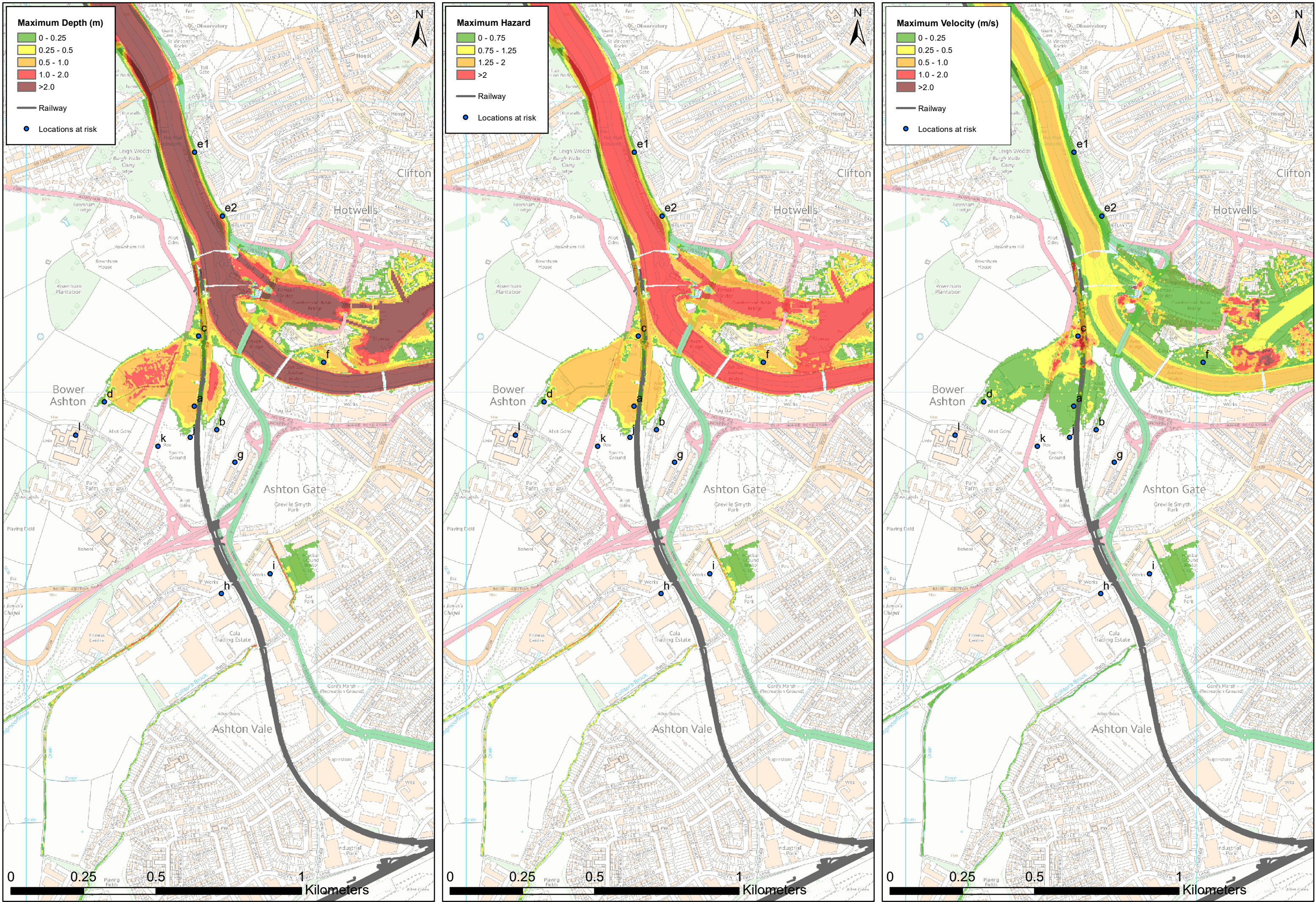
Figure N-16: Post Development, 75year return period event in 2075 ,Tidal
